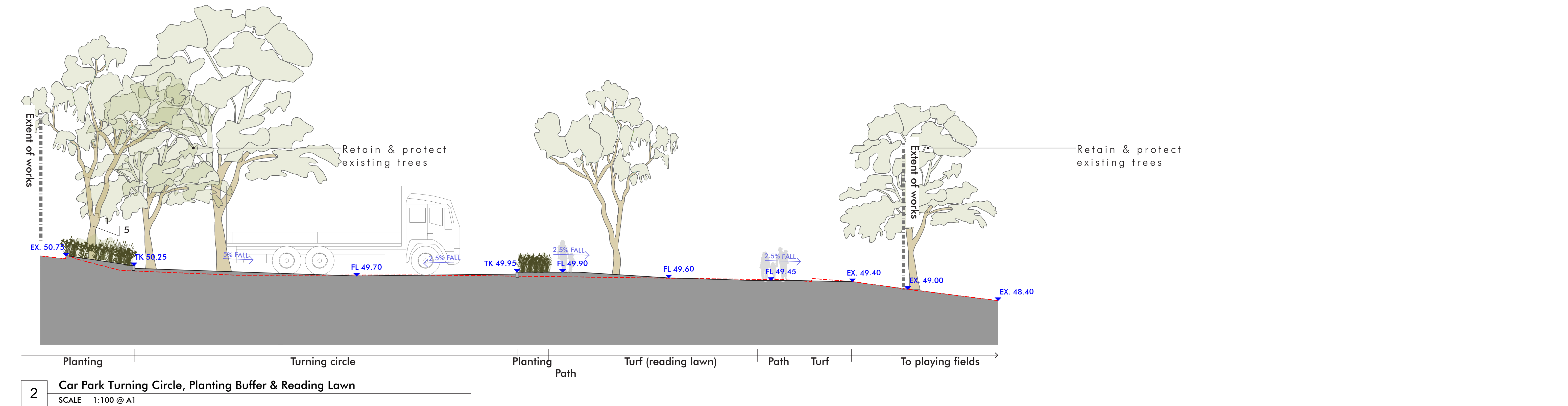
1 Car Park, Planting Buffer & Reading Lawn SCALE 1:100 @ A1
